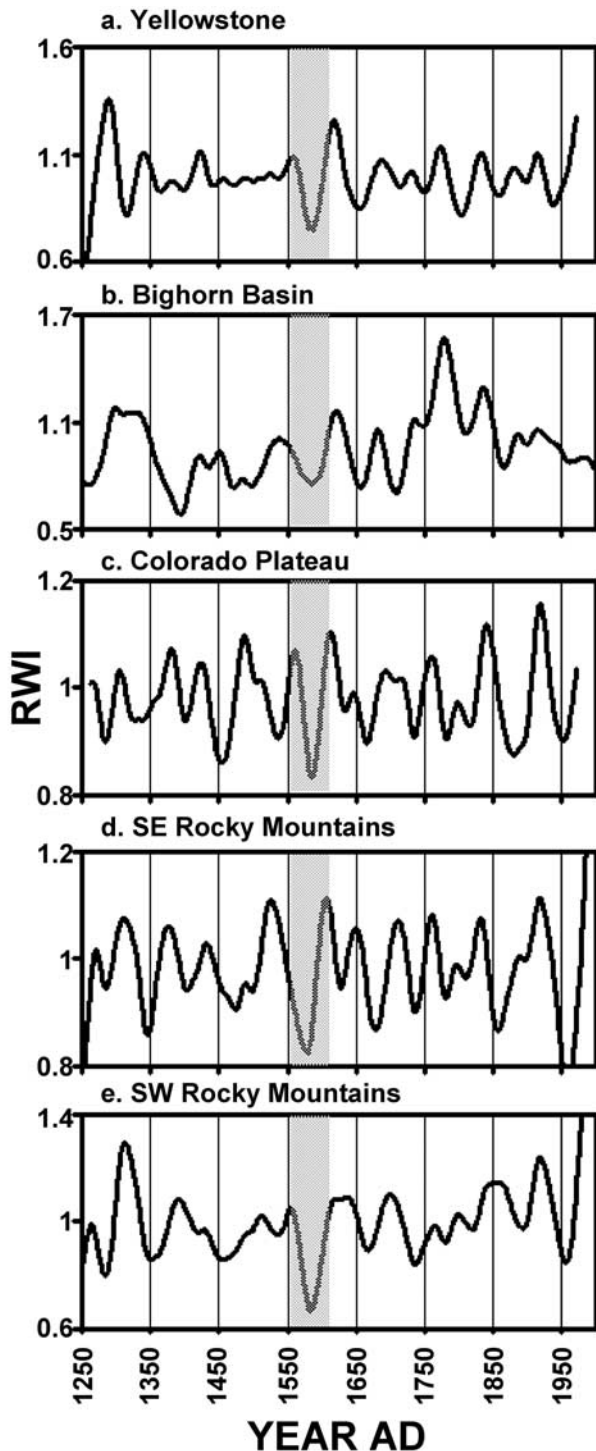
Figure 3. 50-yr smoothed ring-width index (RWI) values for the regional composite chronologies. Gray shading represents the late 16th century megadrought of Woodhouse and Overpeck [1998] and Stahle et al. [2000]. Smoothed values were produced by applying a cubic spline set to capture 50% of the variance at a wavelength of 50 years.
