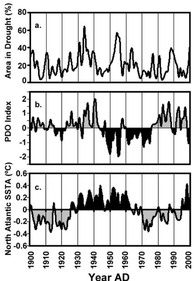
Figure 4. (a) Annual plot showing % of contiguous United States experiencing drought conditions ( PDSI < -2 ). (b) Plot of average annual Pacific Decadal Oscillation (PDO) index values [ Mantua and Hare , 2002]. (c) Detrended sea surface temperature anomalies (SSTA) for the Atlantic Ocean from 0–70° North. The Atlantic Multidecadal Oscillation (AMO) index is a ten-year running mean of this annual series [ Enfield et al. , 2001].
