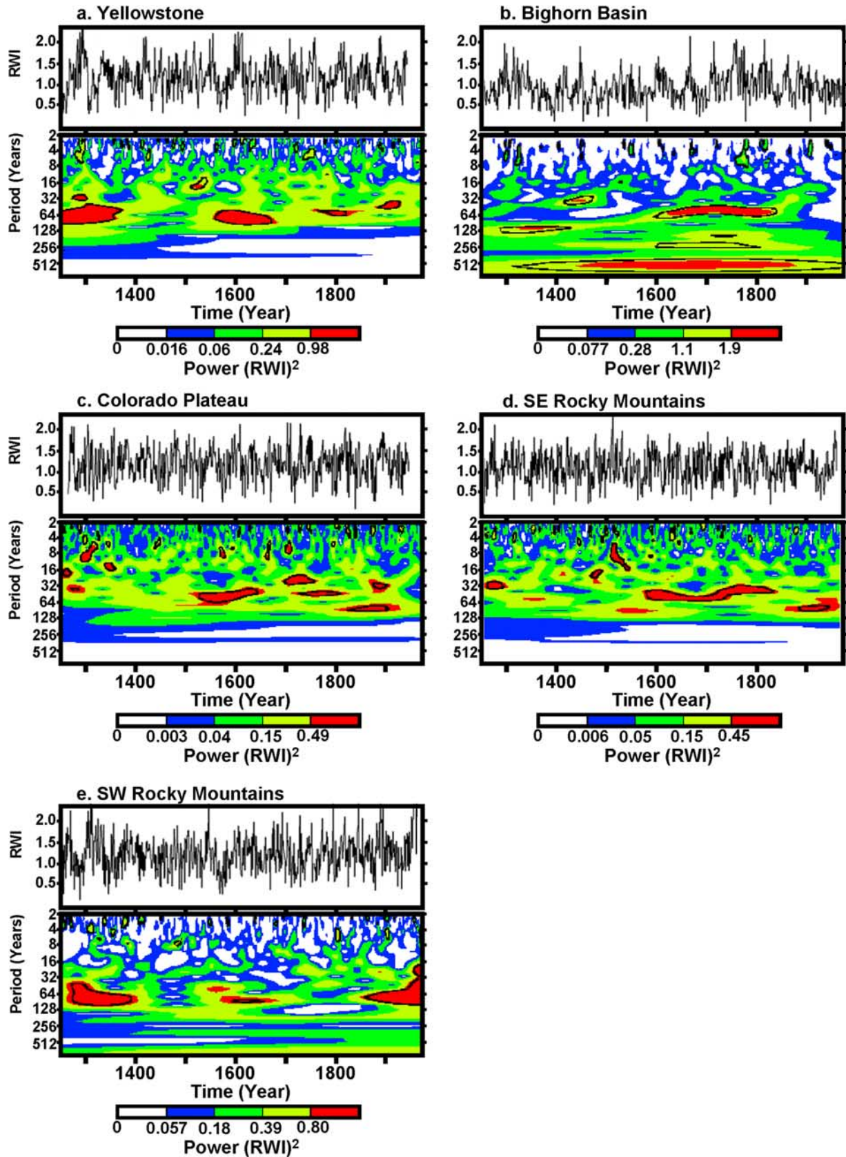
Figure 2. Plots of average ring width index (RWI) values (top) and wavelet power spectra (bottom) for the regional composite chronologies. The colored contour intervals represent 75, 50, 25, and 5% of the wavelet power, respectively. Black contours in the wavelet power spectra represent the 95% confidence level using a red-noise background spectrum. All analyses employed the Morlet wavelet and zero-padded series [Torrence and Compo, 1998].
